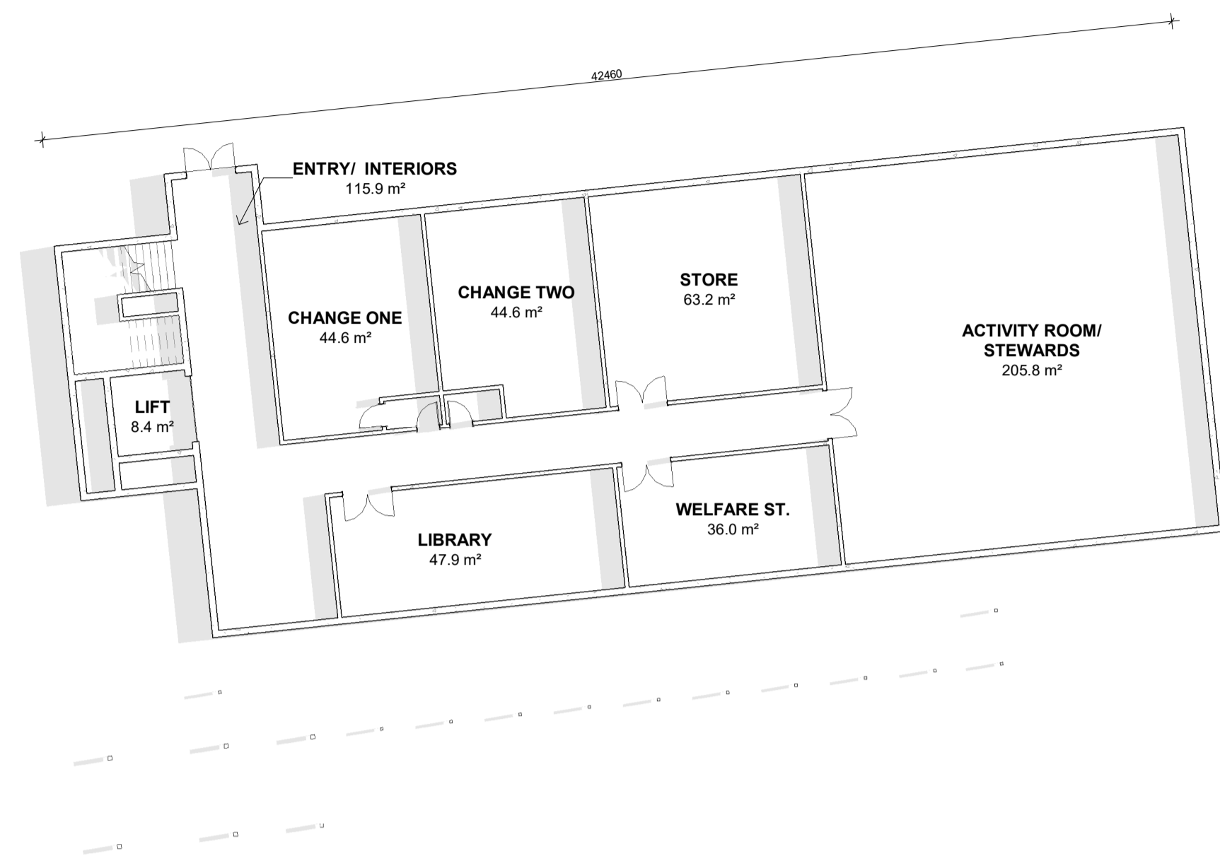
1 TURF - MULTIFUNCTION GROUND SCHEMATIC 1 : 200
